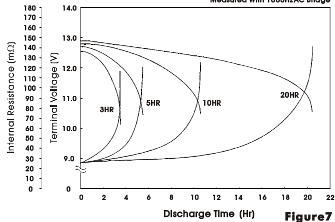
Figure7. INTERNAL RESISTANCE OF BP BATTERY
