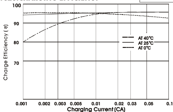
Figure23. CHARGING EFFICIENCY
