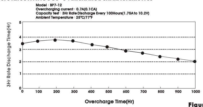
Figure12. CONTINUOUS OVERCHARGE CHARACTERISTICS
